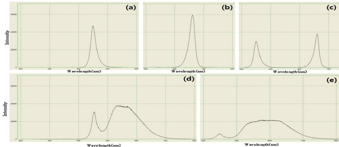
[Fig. 1] Emission spectra of LED using in this study.
